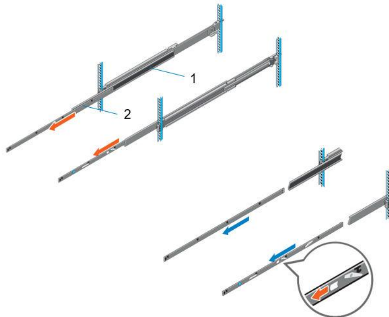
Figure 37. Pull out the intermediate rail
