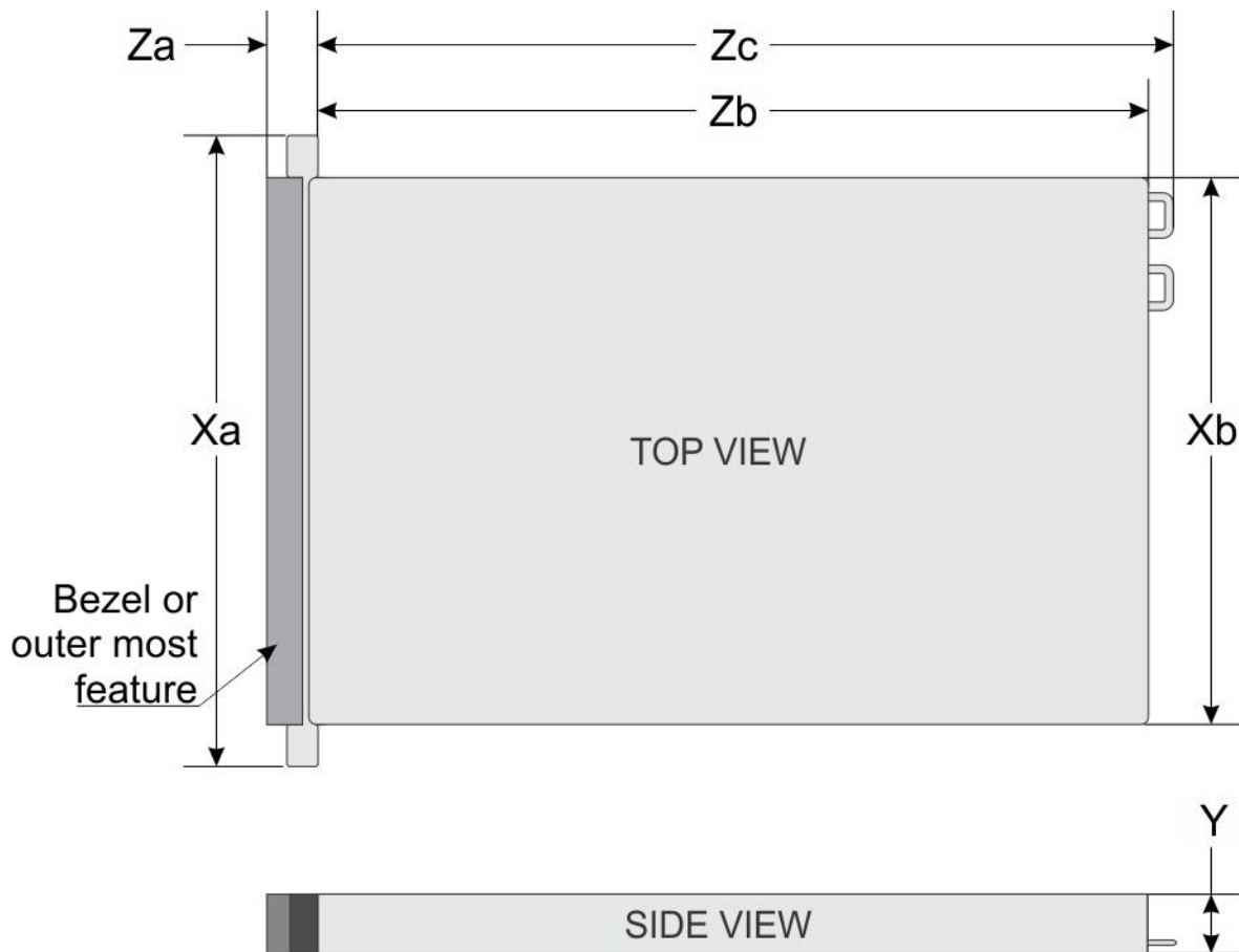
Figure 41. Chassis dimensions
