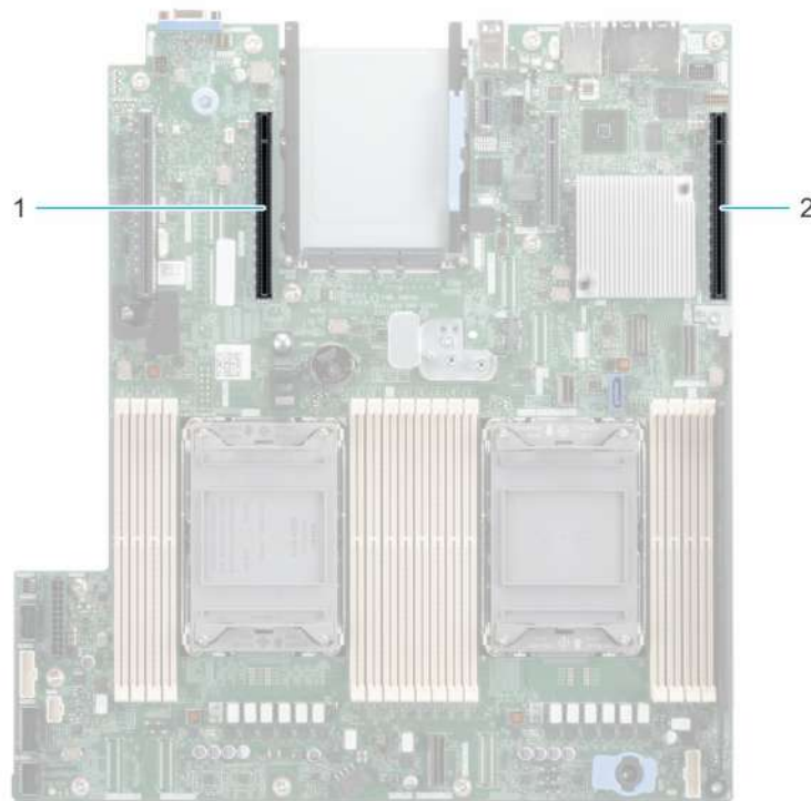
Figure 7. Expansion card slot connectors
